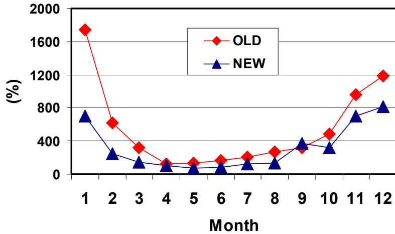
Mean Normalized Bias _ PM25
