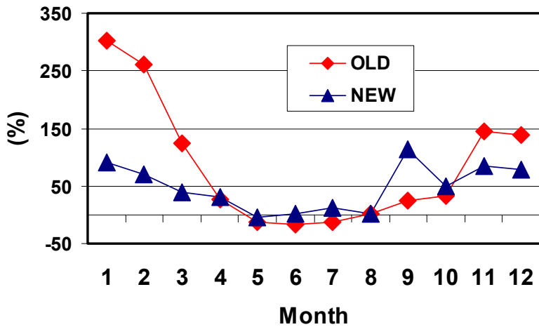
Mean Normalized Bias _ PM25
