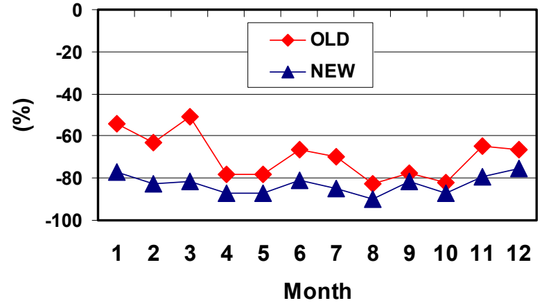
Mean Normalized Bias _ RCFM
