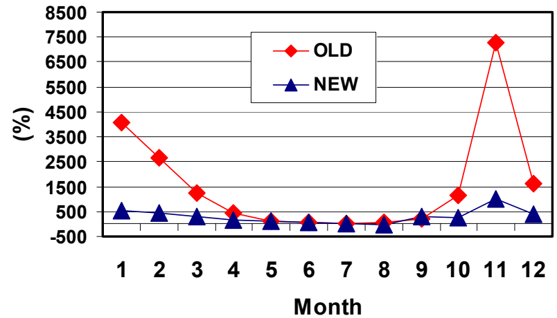
Mean Normalized Bias _ EC
