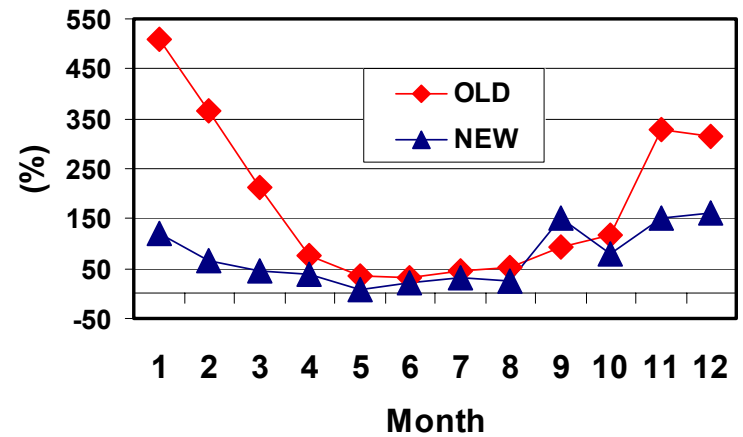
Mean Normalized Bias _ RCFM
