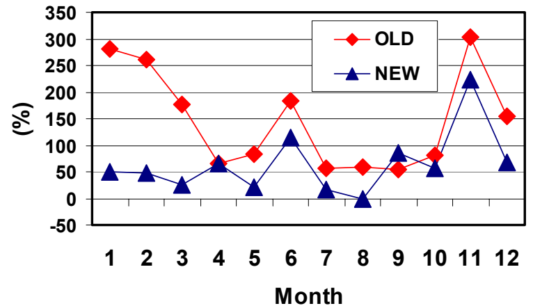
Mean Normalized Bias _ EC
