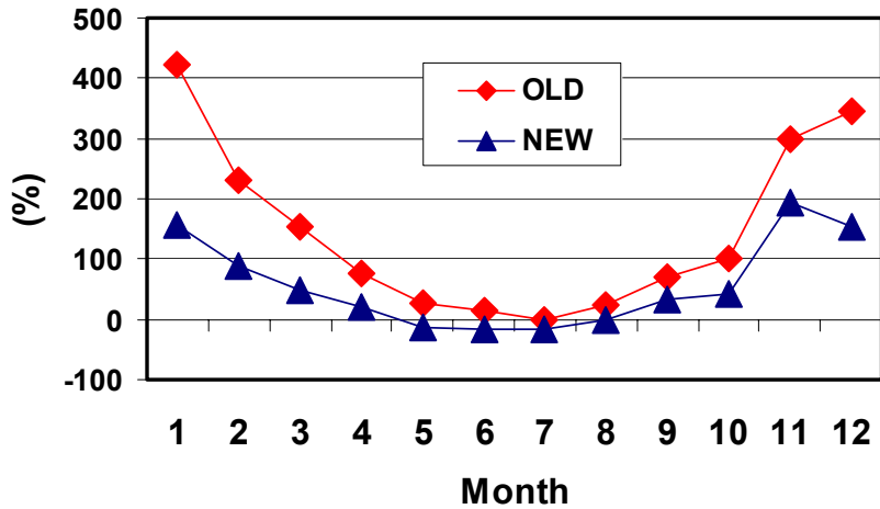
Mean Normalized Bias _ OC
