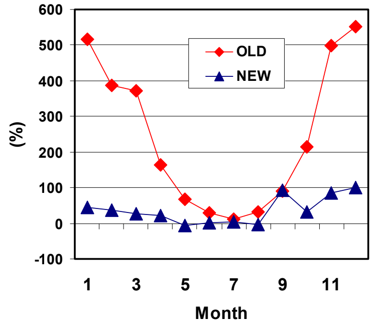
Mean Normalized Bias _ BEXT
