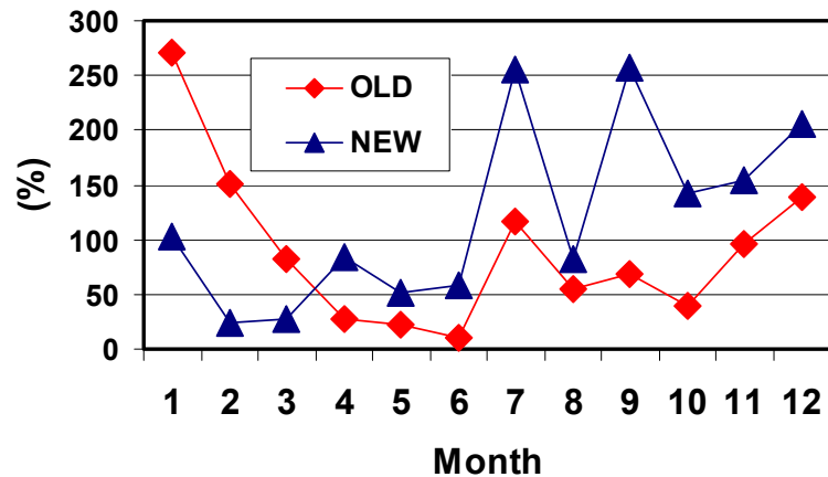
Mean Normalized Bias _ OC
