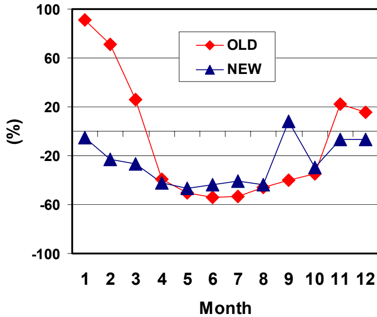
Mean Normalized Bias _ PM10
